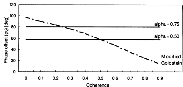
Fig. 4. Mean absolute coherence versus \pm max phase offset caused by the Goldstein (horizontal lines) and modified Goldstein filter (dashed line).
