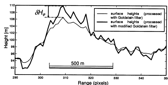
Fig. 8. Cross section over the surface heights.
