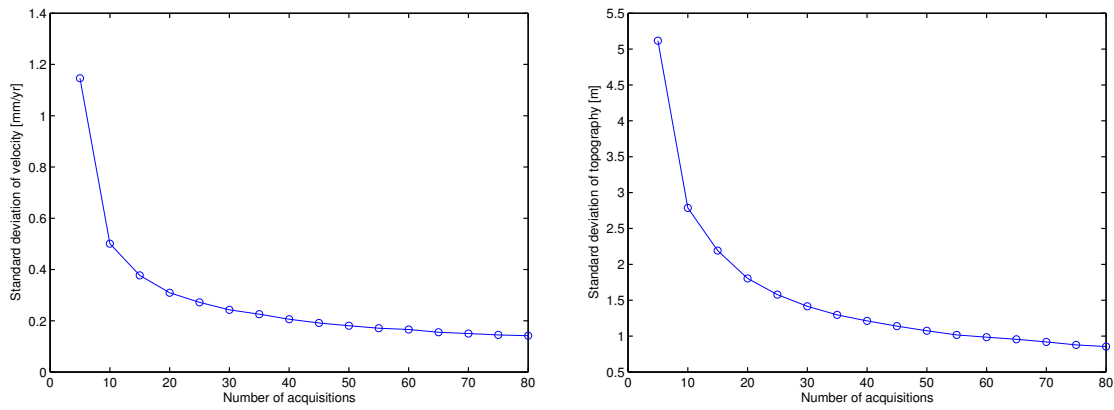
Figure 3: Precision (standard deviation) of estimated deformation and topography as a function of the available images
