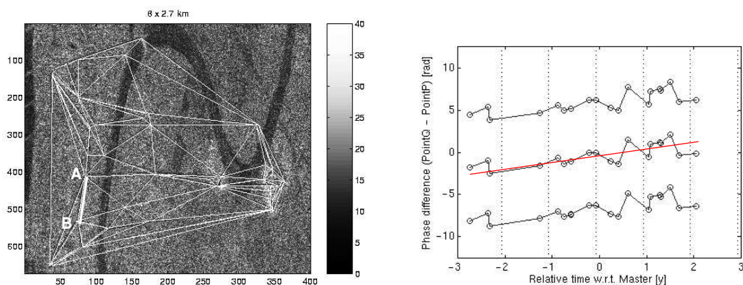
Figure 2: Permanent scatterers example over Hangu, China. A network of opportunity is defined, and the time evolution between two points is shown.
