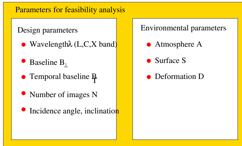
Figure 1: Main parameters influencing the feasibility of deformation monitoring using satellite InSAR.
