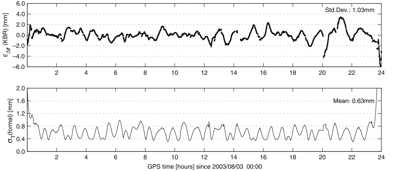
Fig. 3 For 2003 DOY 215: top true GRACE relative position error, \epsilon_{\Delta r} , from the DGPS filter verified using KBR data. Bottom the formal DGPS filter along-track error ( 1\sigma )
