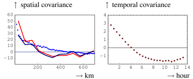
Figure 5: Covariograms of the IWV data. Left: spatial. In dark blue: GPS covariogram at 10:30. In red: mean of 24 hourly spatial GPS covariograms. In blue: covariogram of the MERIS data. Right: temporal. Mean of the 26 temporal covariograms of the detrended IWV values at the different GPS stations.
