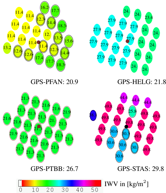
Figure 4: IWV values at 25 MERIS pixels most close to a GPS station. Top left: Pfaender. Top right: Helgoland. Bottom left: Braunschweig. Bottom right: Stavanger. ‘LAND’ pixels are surrounded by one circle, ‘COAST-LINE’ pixels by two circles.
